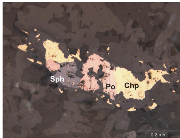
Fig. 3. Pyrrhotite (Po) with chalcopyrite (Chp) and sphalerite (Sph) in wollastonite matrix.
